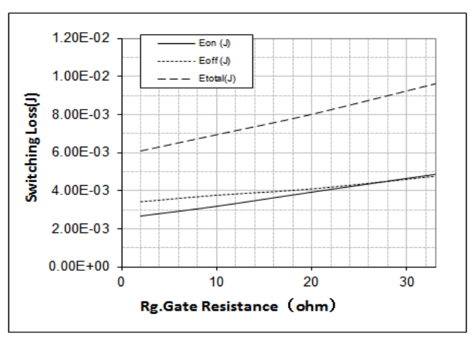
Switching Loss vs. Rg(175°C)
