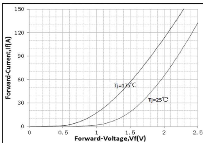
Diode Characteristic
